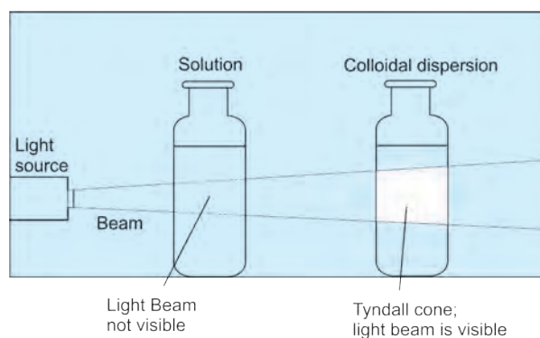
Fig. 11.8 :Tyndall effect
